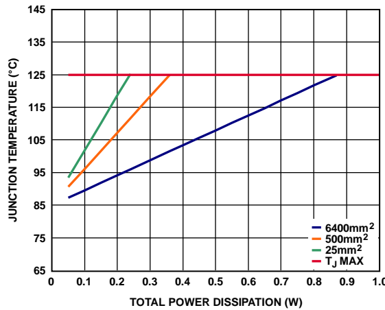
Figure 75. SOIC, T_A = 85^\circ\text{C}
