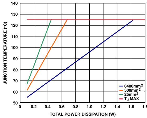
Figure 74. SOIC, T_A = 50^\circ\text{C}
