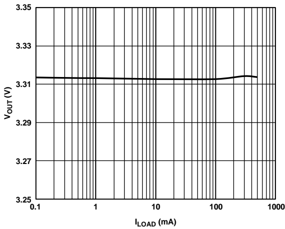
Figure 6. Output Voltage vs. Load Current
