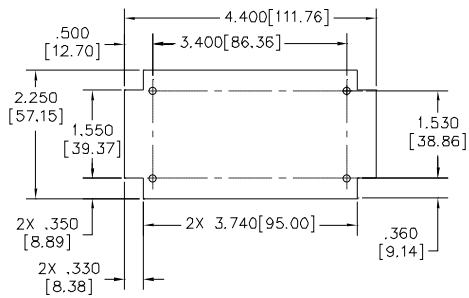
MAXIMUM PCB DIMENSIONS BOTTOM COVER MTG.
