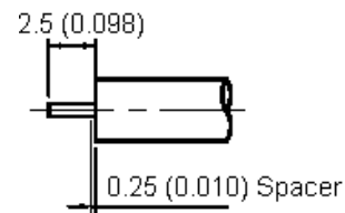
Stripping Dimension
