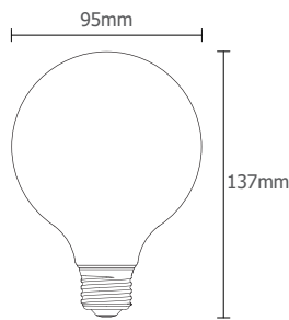
G95F8-M-D-8.5W-E-E27
