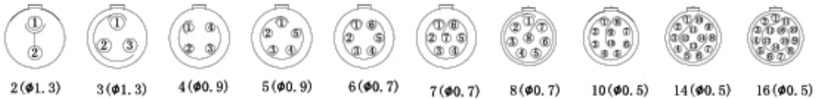
CONNECTOR SOLDER CUP VIEW
