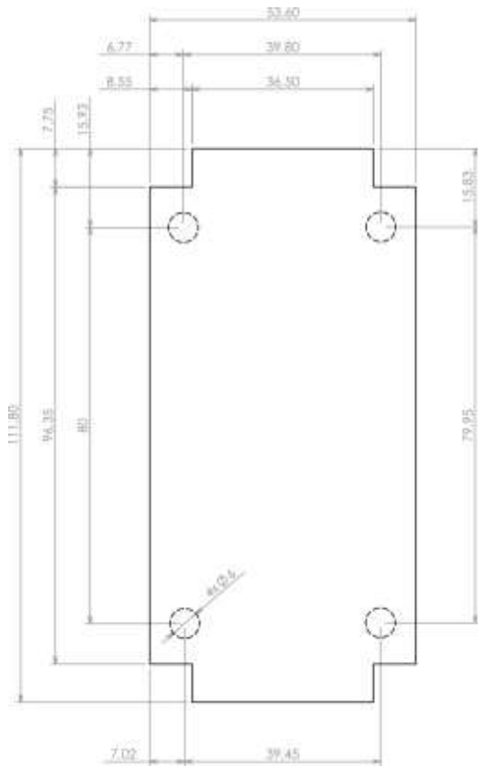
Base PCB
