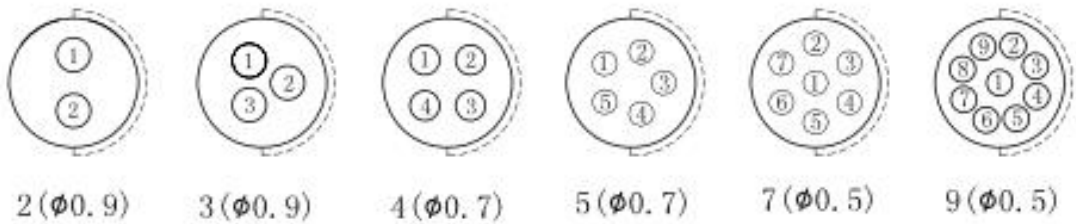
CONNECTOR SOLDER CUP VIEW
