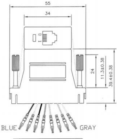
DB25 PIN FEMALE TO 8P8C
