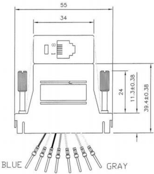
DB25 PIN MALE TO 8P8C
