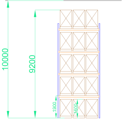
Front View – 5 Levels (10m)
