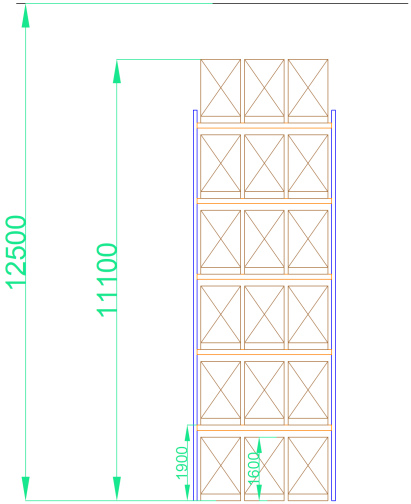
Front View – 6 Levels (12.5m)
