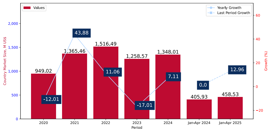
Figure 4. United Kingdom's Market Size of Seats with wooden frames, upholstered in M US$ (left axis) and Annual Growth Rates in % (right axis)
