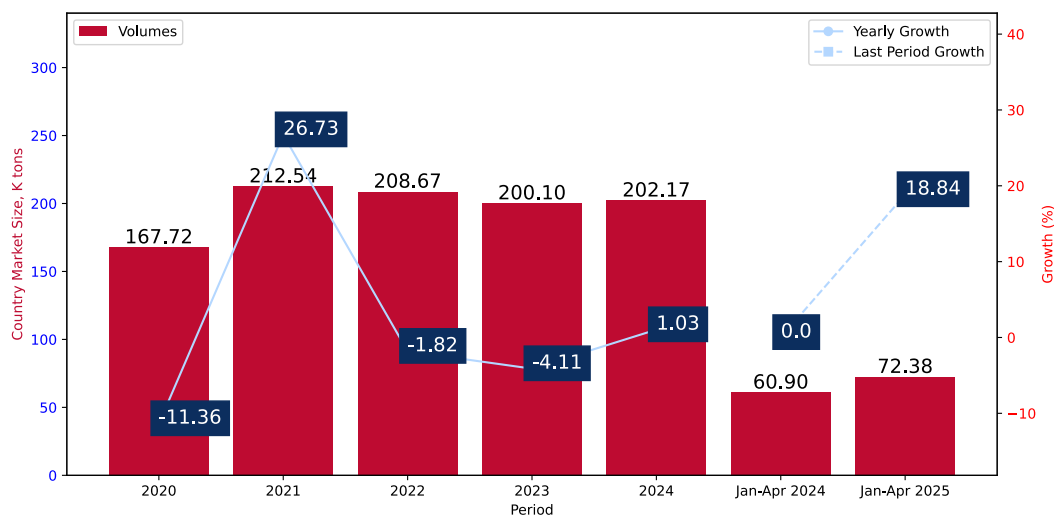
Figure 5. United Kingdom's Market Size of Seats with wooden frames, upholstered in K tons (left axis), Growth Rates in % (right axis)
