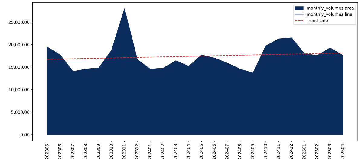
Figure 9. Monthly Imports of United Kingdom, tons 0.35% 4.32% monthly annualized
