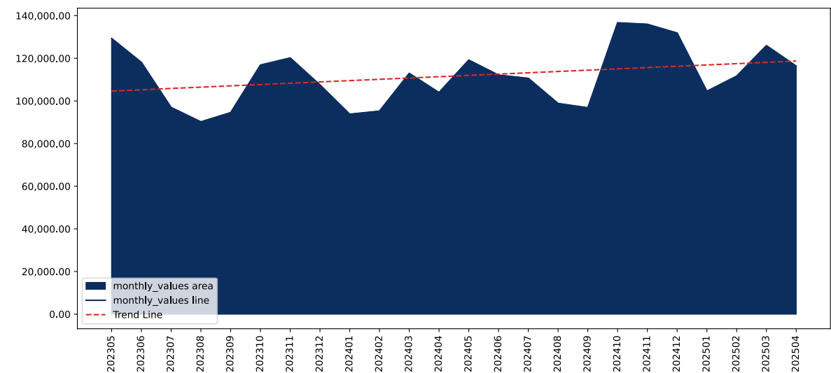
Figure 7. Monthly Imports of United Kingdom, K current US$ 0.55% 6.81% monthly annualized
