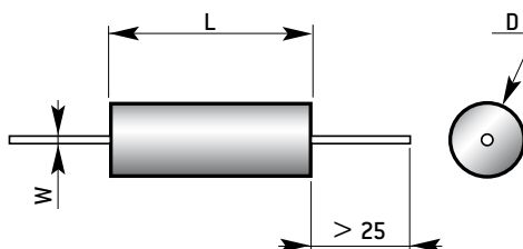
Axial leads Model RA 75
