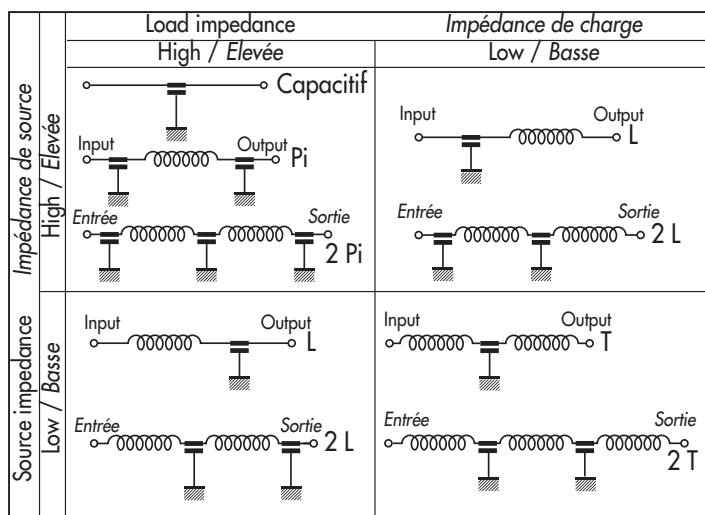
Filter structures
