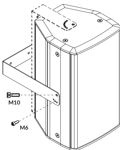
VERTICAL INSTALLATION
