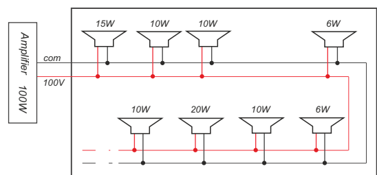
AFTER Speakers were added and removed from the system. The total requested power is now 87W. In this case it is sufficient to change the amplifier, but the system (in terms of cables) will remain unaltered.
