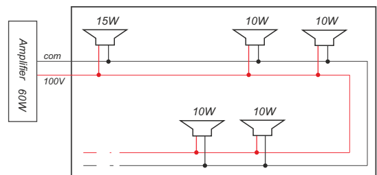
BEFORE 5 speakers were connected to the system for a total of 55W. The selected amplifier was 60W.
