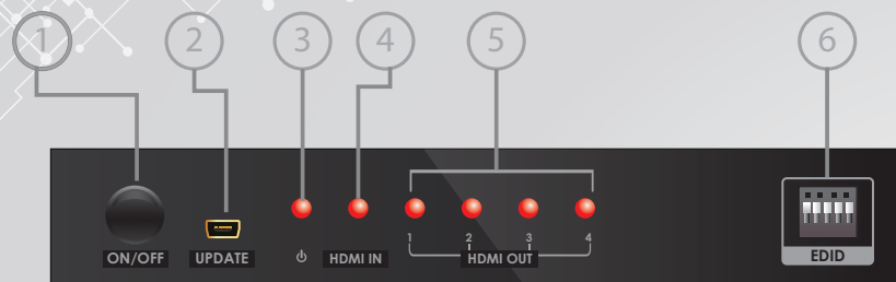
Front Panel
