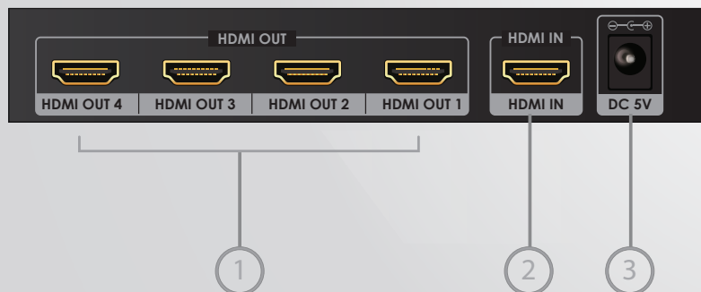
Rear Panel
