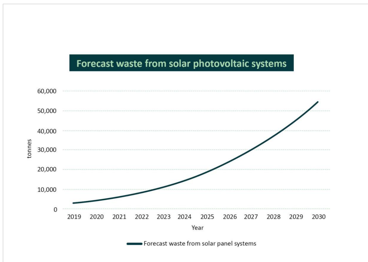
Graph 1: Forecast waste from solar photovoltaic systems
