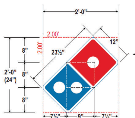
A Domino's Tile Logo Raceway 24" SCALE: 1 1/2" = 1'-0" QTY: ONE (1) AREA: 4.0 SQ. FT.
