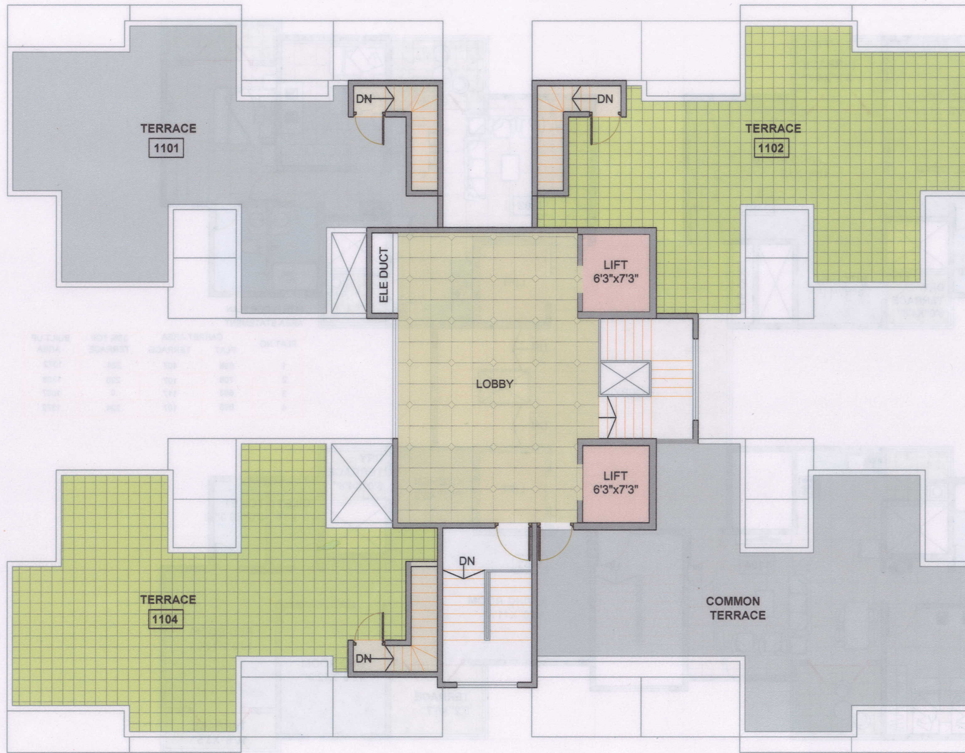
WING E2 - TERRACE FLOOR PLAN
