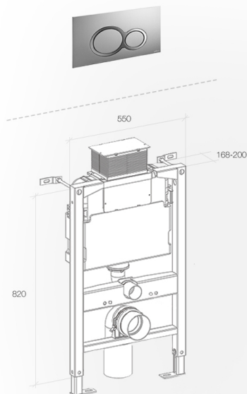
VOLE CHROME DANZA DZ3300-CP XL2001/8041 CONSTELLATION WALL HUNG CISTERN & FRAME
