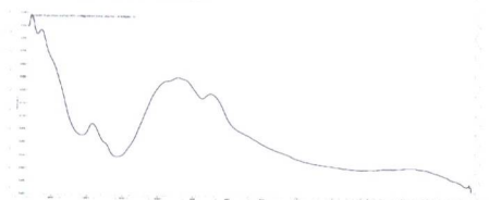
Ultraviolet-visible spectroscopy
