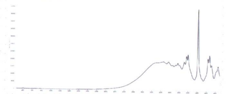
Ultraviolet-visible spectroscopy
