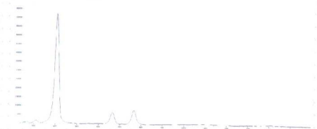
Photoluminescence
