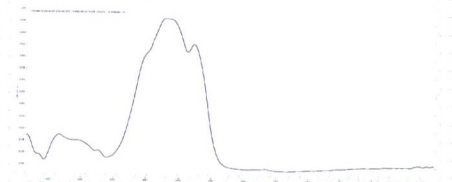
Ultraviolet-visible spectroscopy
