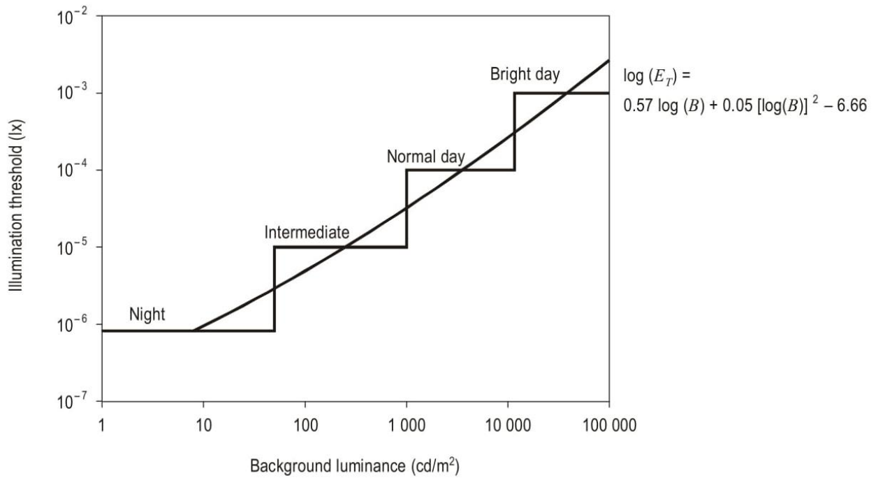
Figure D-1 Relationship between the illumination threshold E_T ( \text{lx} ) and background luminance B ( \text{cd/m}^2 )
