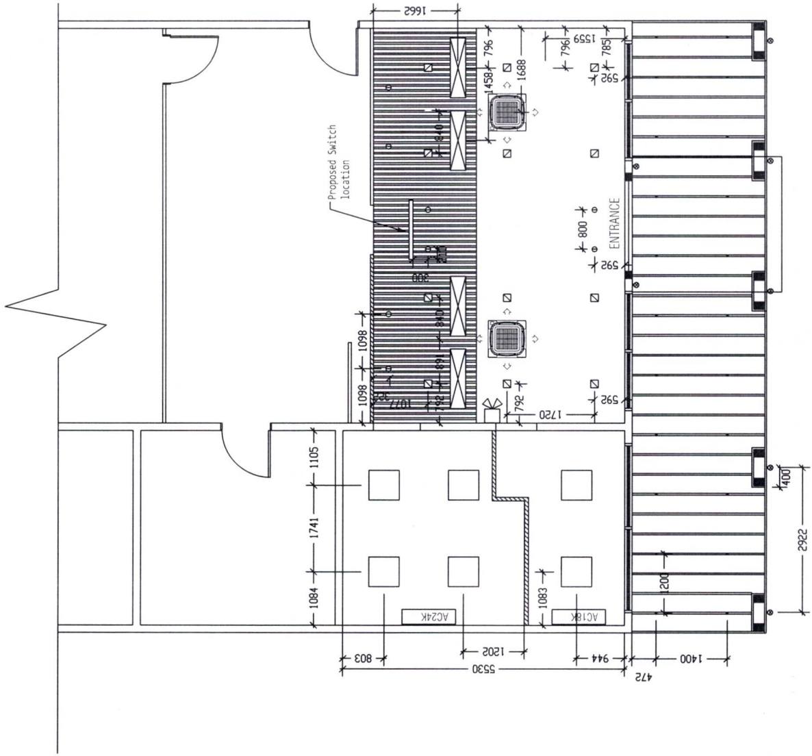
LIGHTING PLAN SCALE: 1:100
