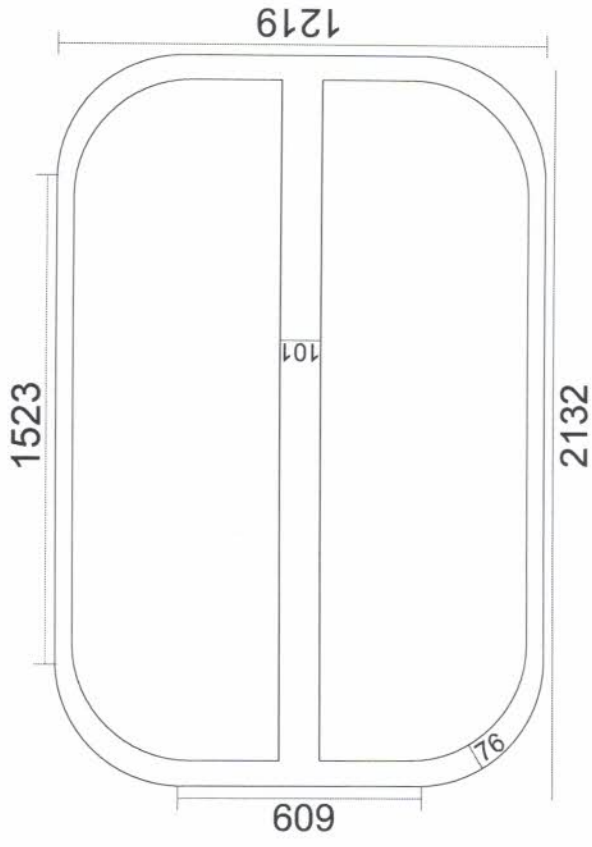
Fish Cutting Board top elevation
