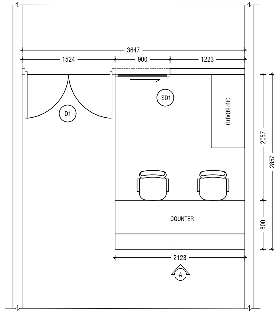
FUNITURE LAYOUT PLAN
