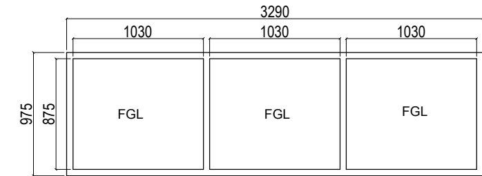
FRAME - C DETAIL
