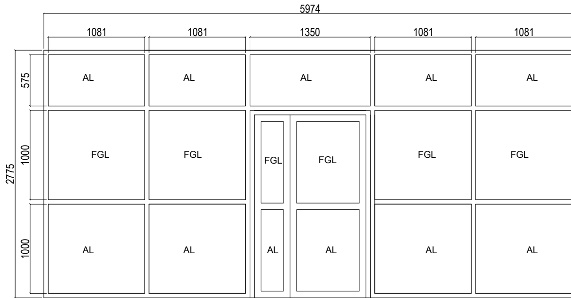
FRAME - A DETAIL
