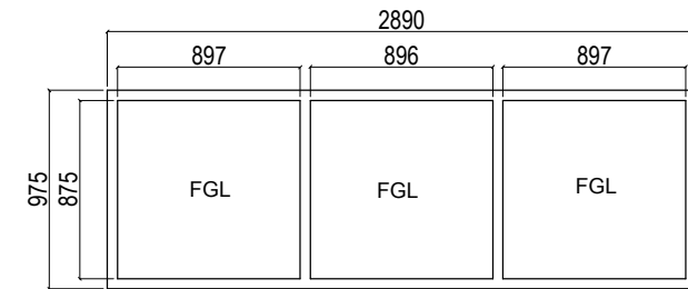
FRAME - C DETAIL
