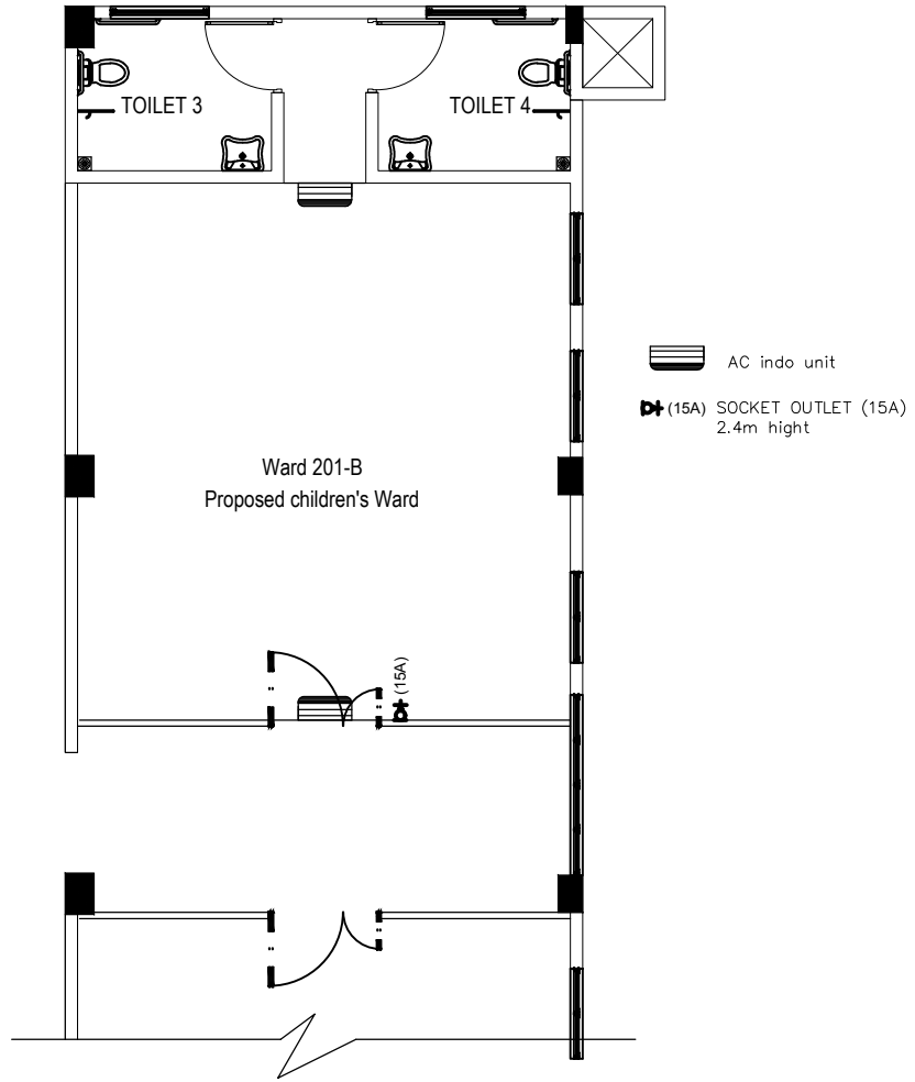
AC & Electric PLAN
