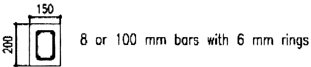
TOP BEAM
