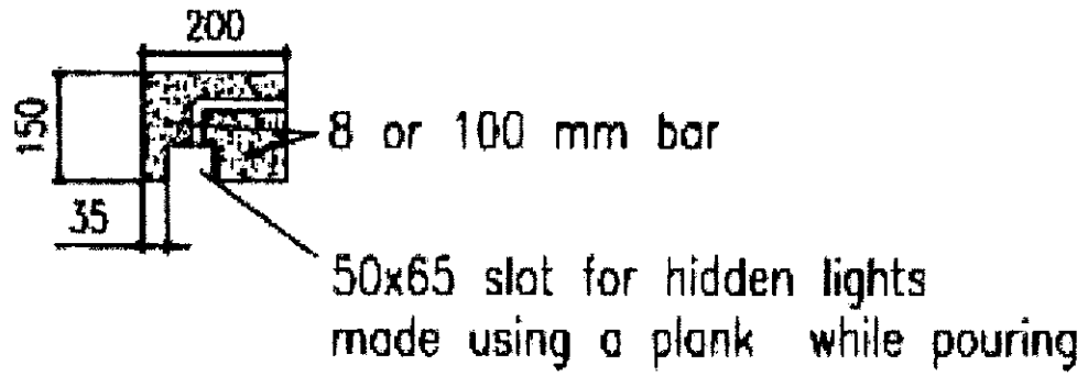
TOP BEAM
