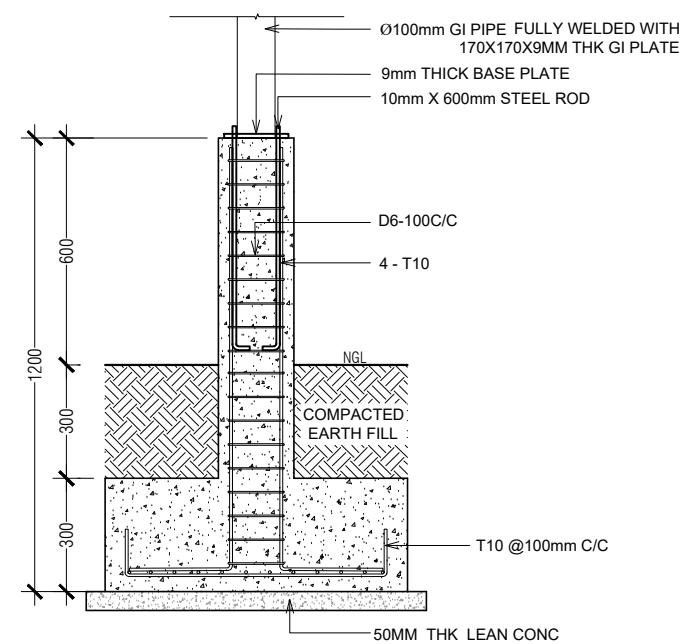
FOOTING SECTION (F1)
