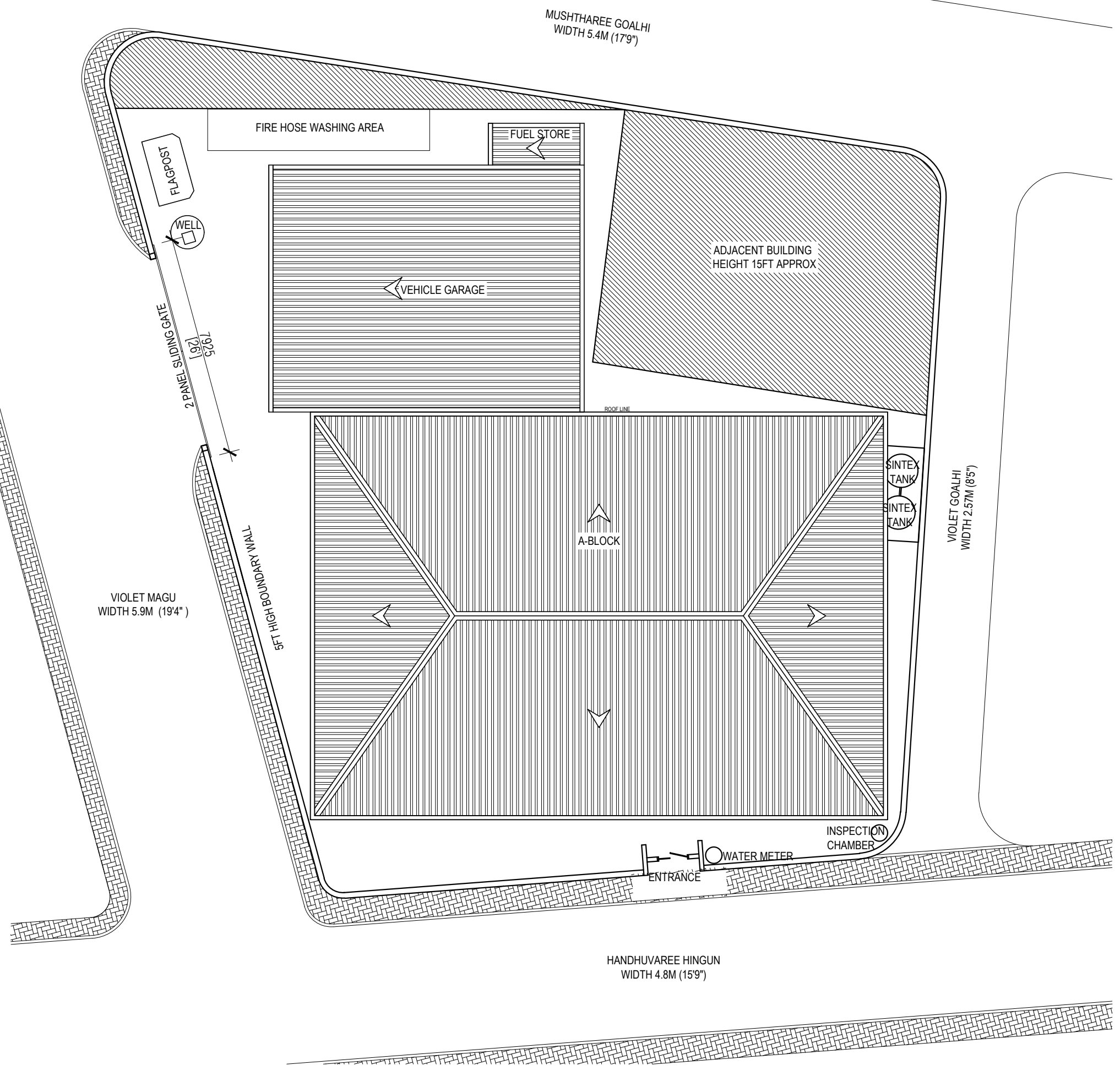
FRS SUBSTATION SITE PLAN (HA. DHIHDHOO) SCALE 1:150
