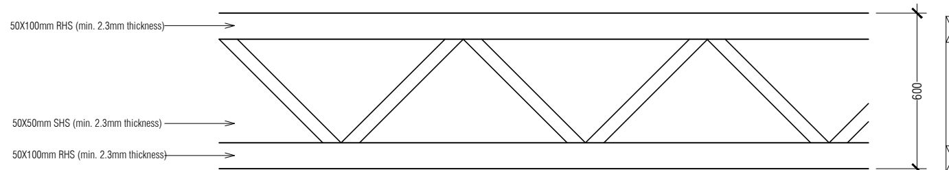
ROOF TRUSS DETAILS (TR2)
