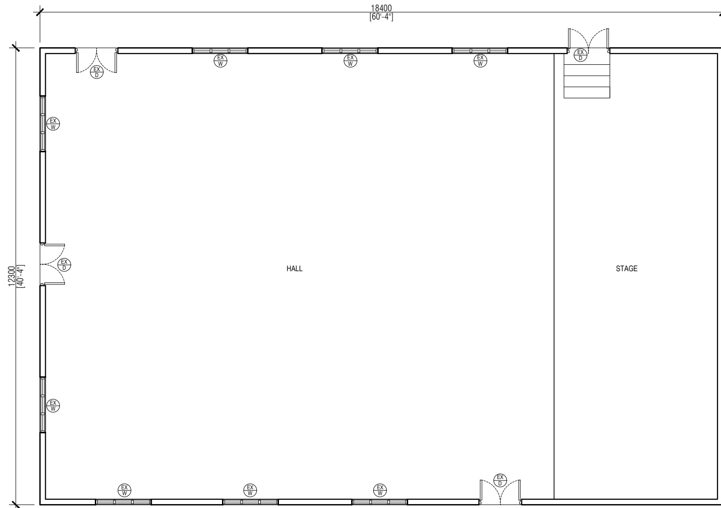
EXISTING FLOOR PLAN SCALE 1:100
