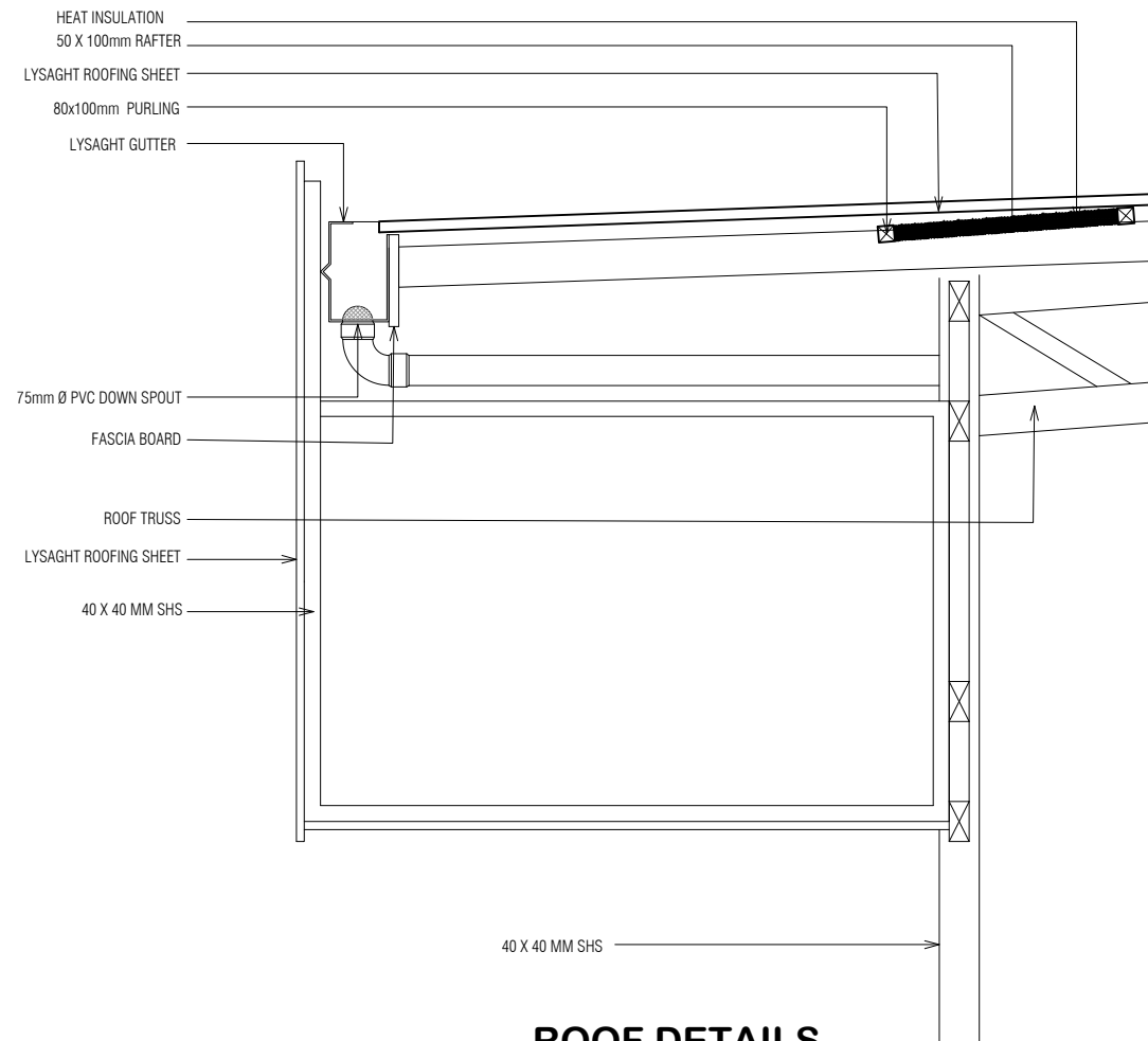
ROOF DETAILS
