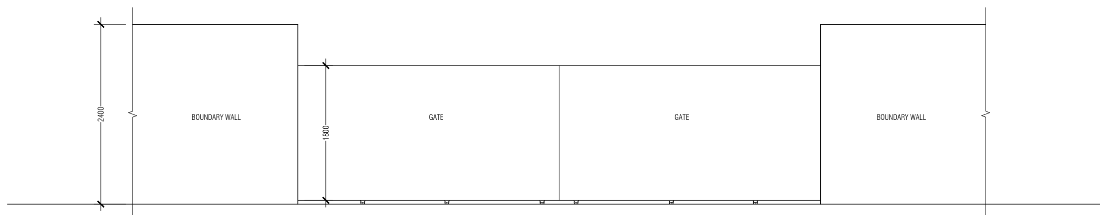
GATE FRONT ELEVATION SCALE 1:50
