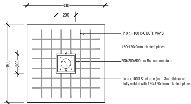
FOOTING PLAN (F1)
