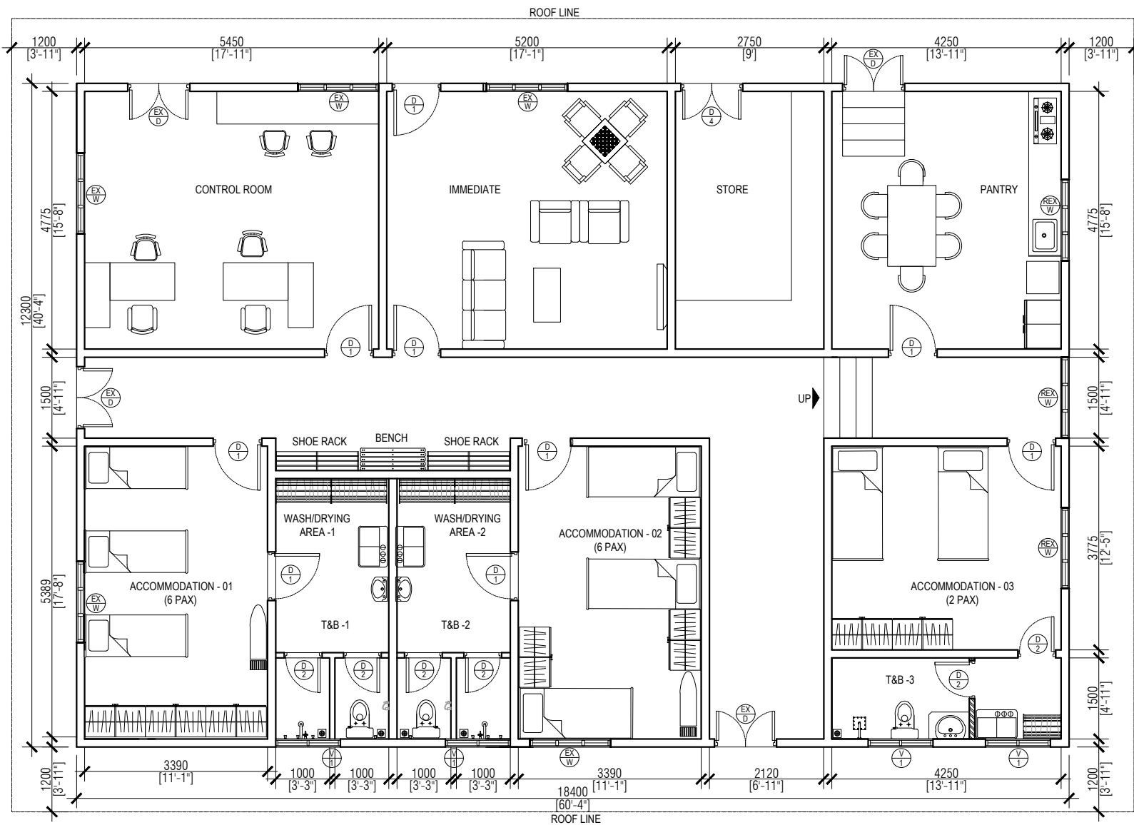
PROPOSED FLOOR PLAN SCALE 1:100
