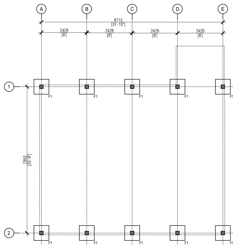
FOOTING & COLUMN PLAN SCALE 1:100
