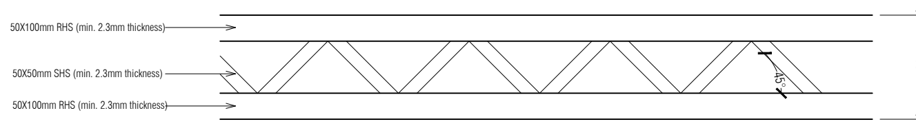
ROOF TRUSS DETAILS (TR1)
