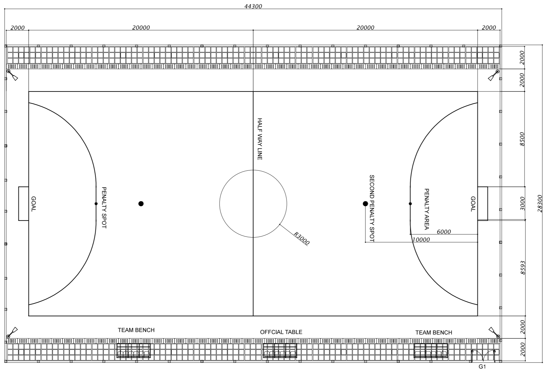
FUTSAL PICH PLAN Scale - 1:200
