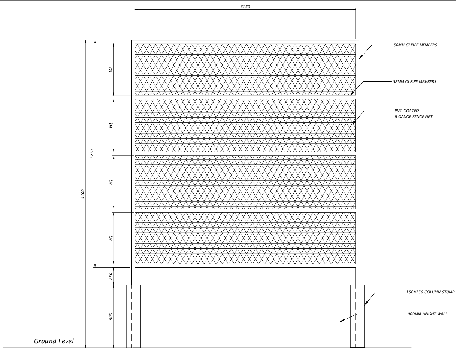
DETAL-PVC FENCE Scale - 1:20
