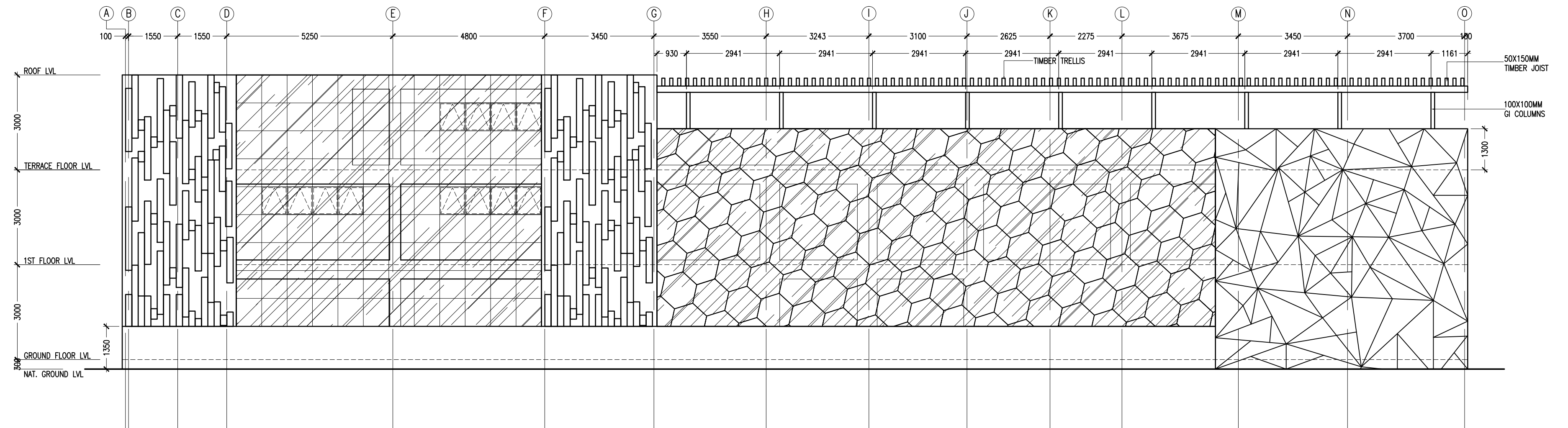
ELEVATION 2 SCALE 1:100
