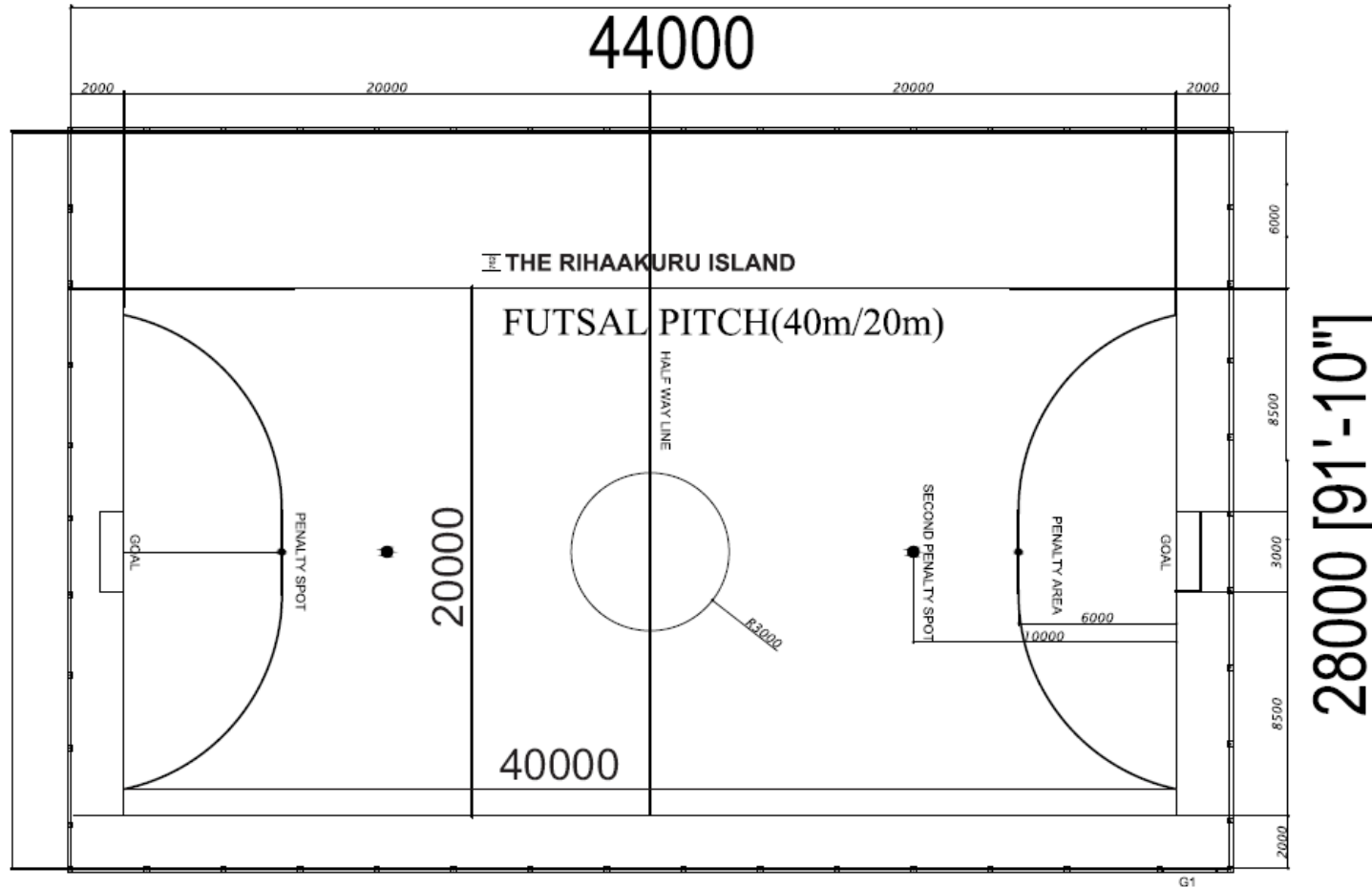
FUTSAL PITCH PLAN Scale - 1:200
