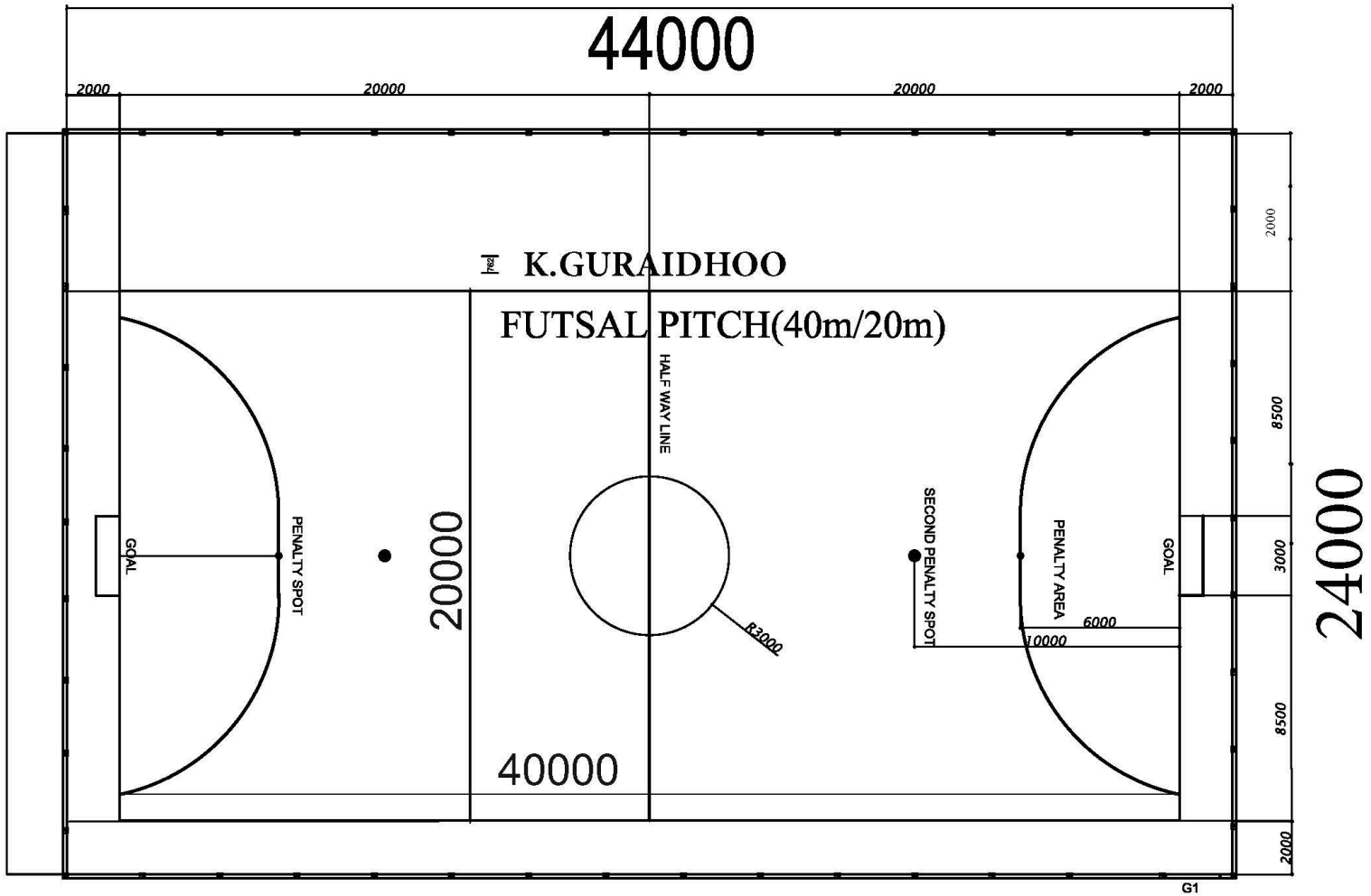
FUTSAL PICH PLAN Scale - 1:200
