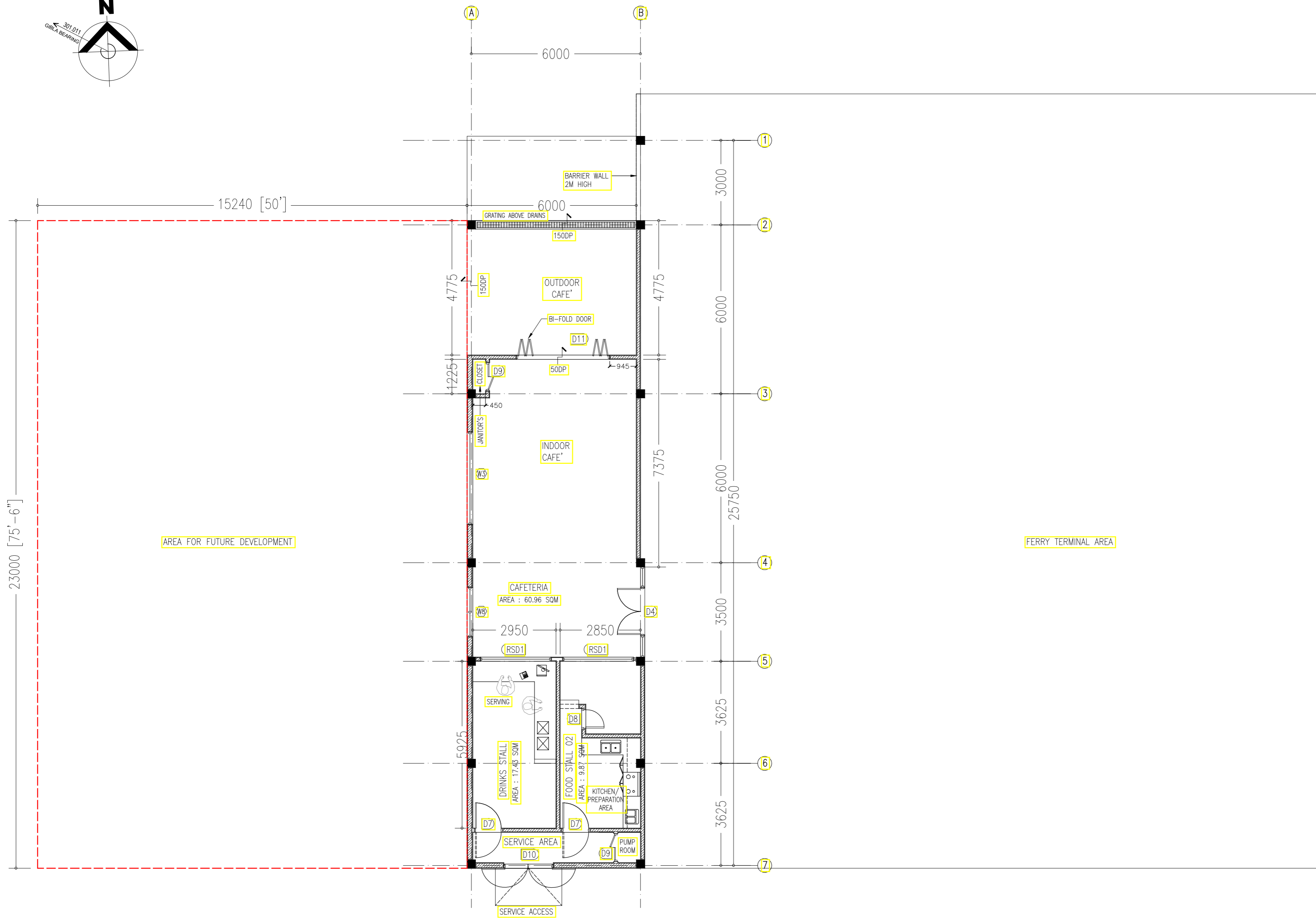
FERRY TERMINAL CAFETERIA (As-built drawing) SCALE: 1:100
