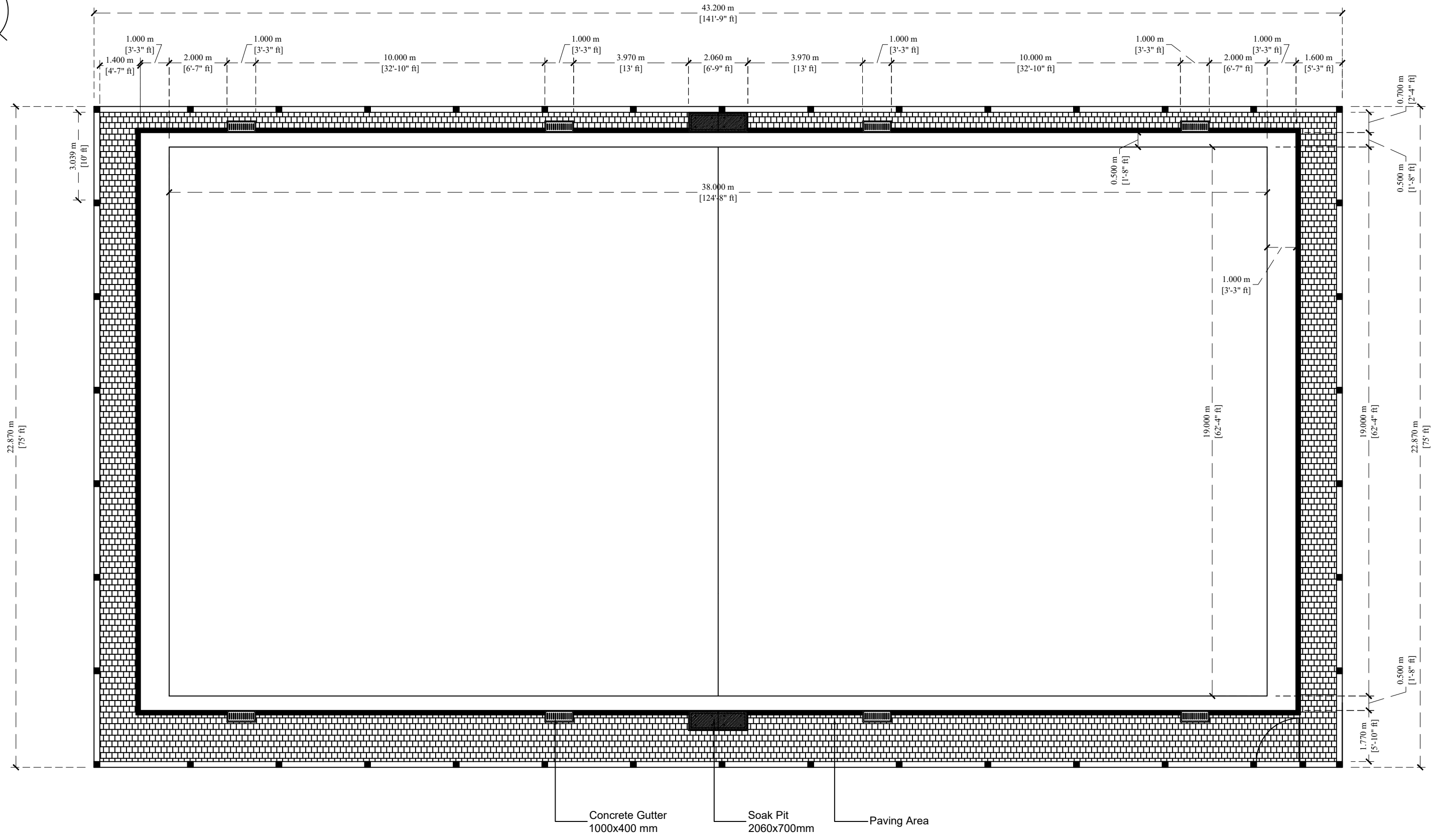
ARTIFICIAL TURF FULL PITCH PLAN
