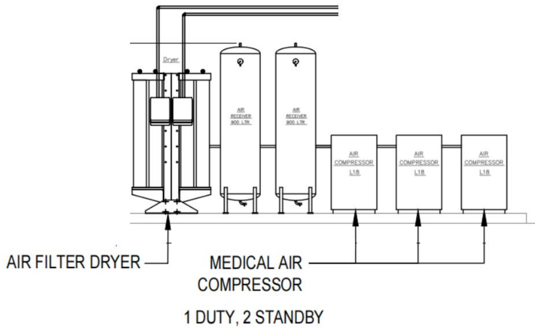
Schematic diagram of medical gas plant
