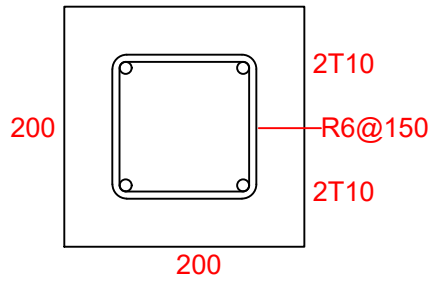
TOP BEAM
