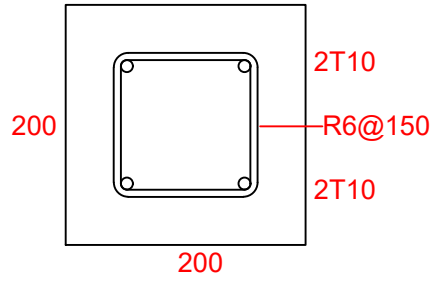
FOUNDATION BEAM
