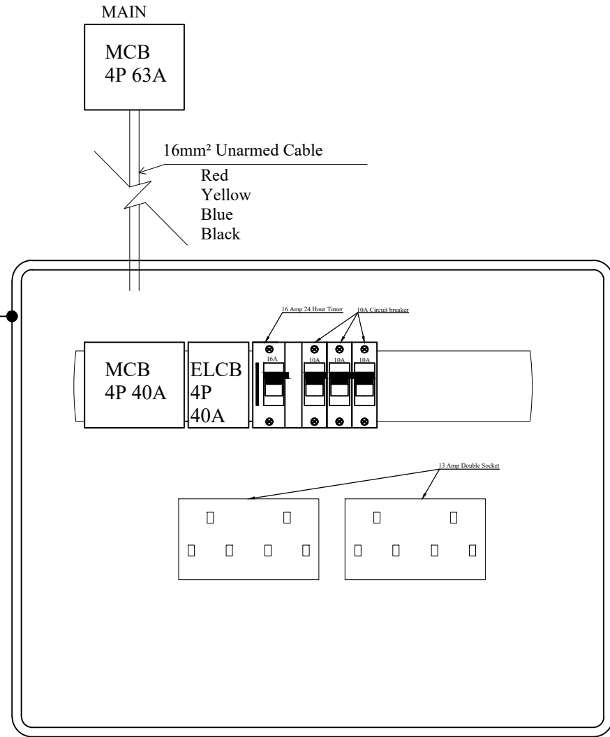
Outdoor DB and Main Cable Cable Diagram
