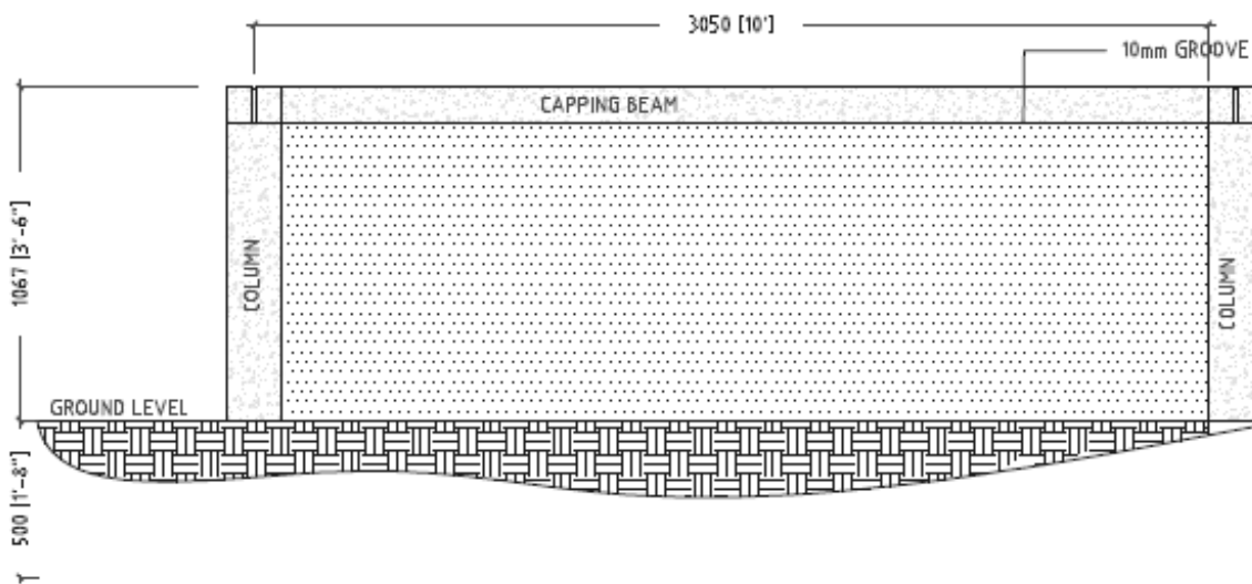
ELEVATION SCALE 1:25
