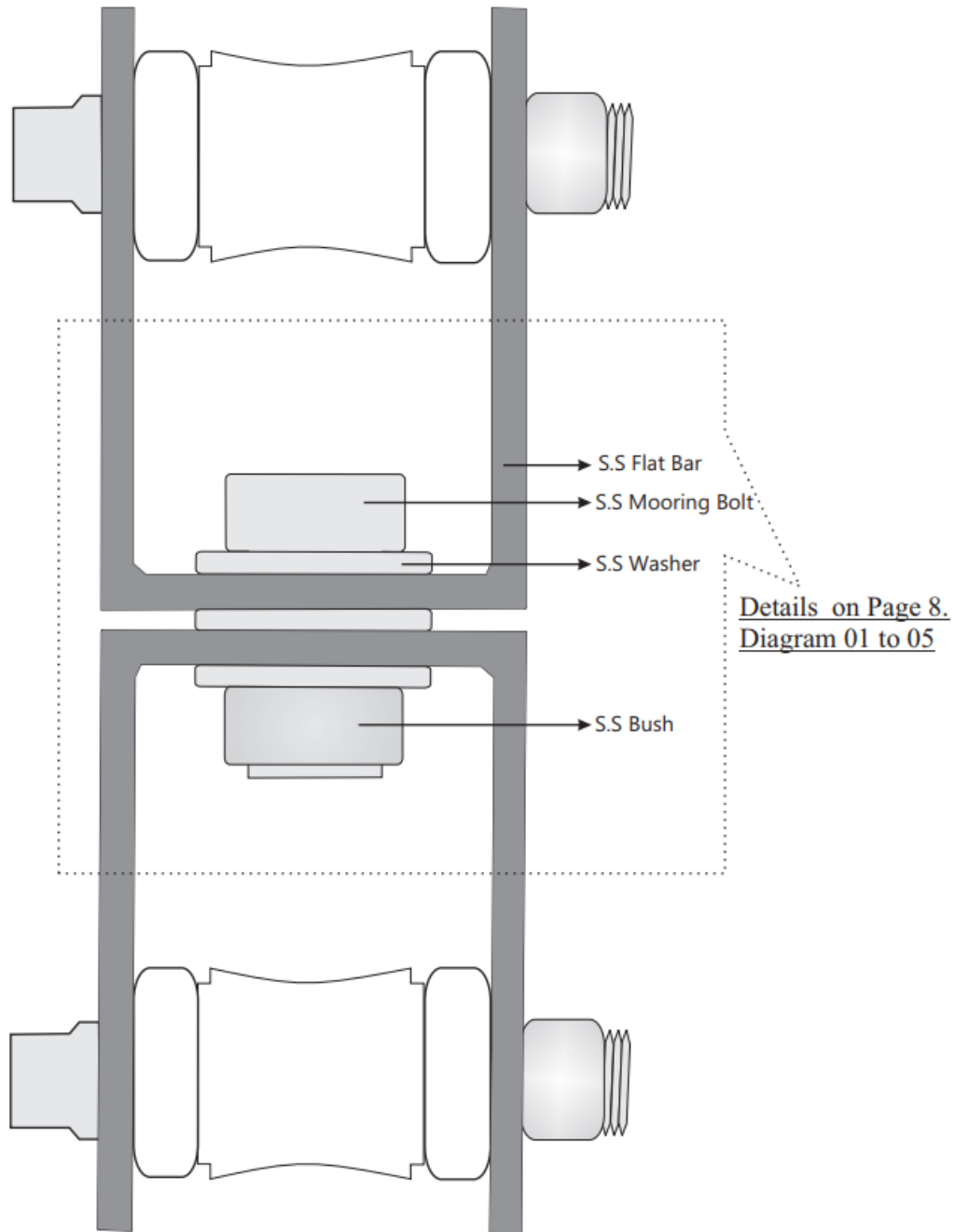
Front view
