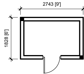
Foundation Plan
