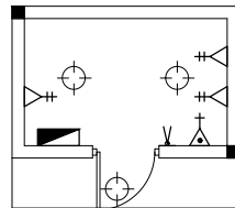
Electric Plan
