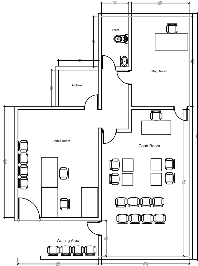
FULIDHOO COURT EXISTING FLOOR PLAN SCALE :1200
