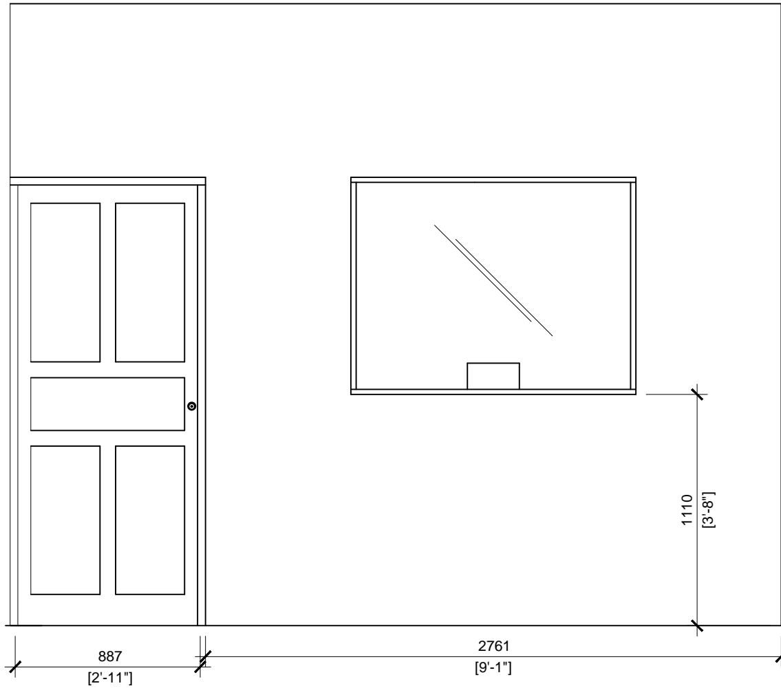
Counter Front View
