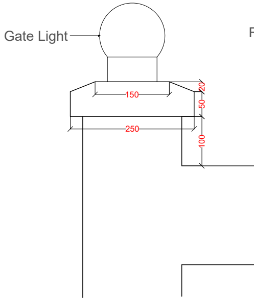
Gates Column Design
