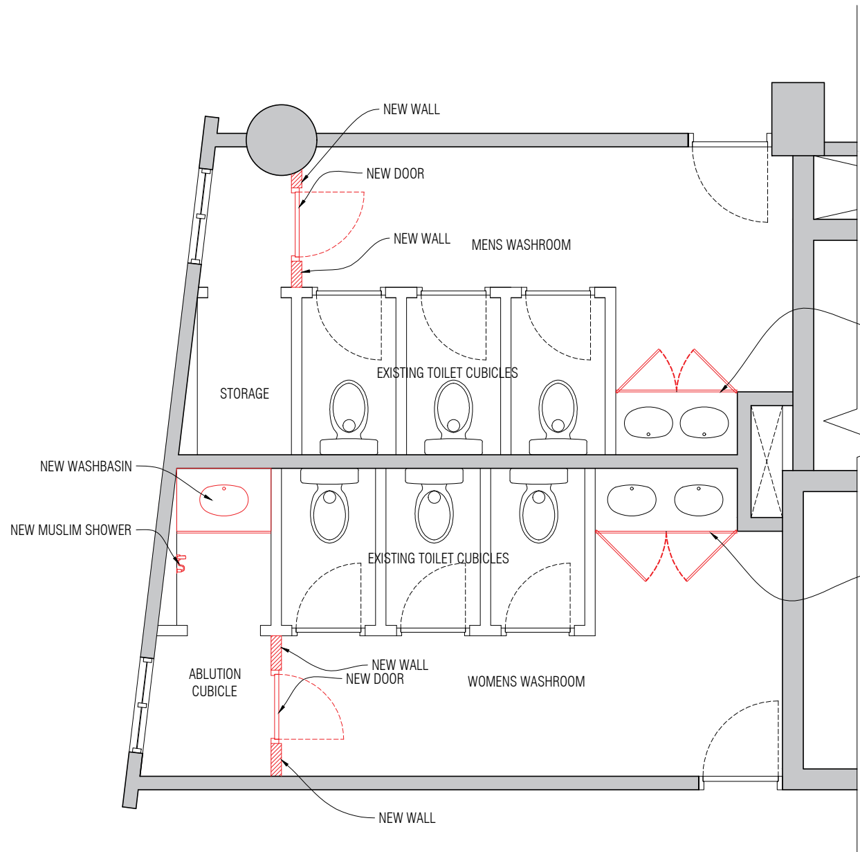
01 GENERAL TOILET LAYOUT A01 SCALE 1:50 0 0.5m 1m 1.5m 2m
