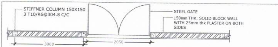
MAIN ENTRANCE GATE DETAIL (PLAN) SCALE 1:50
