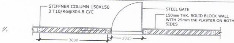
MAIN ENTRANCE GATE DETAIL (PLAN) SCALE 1:50
