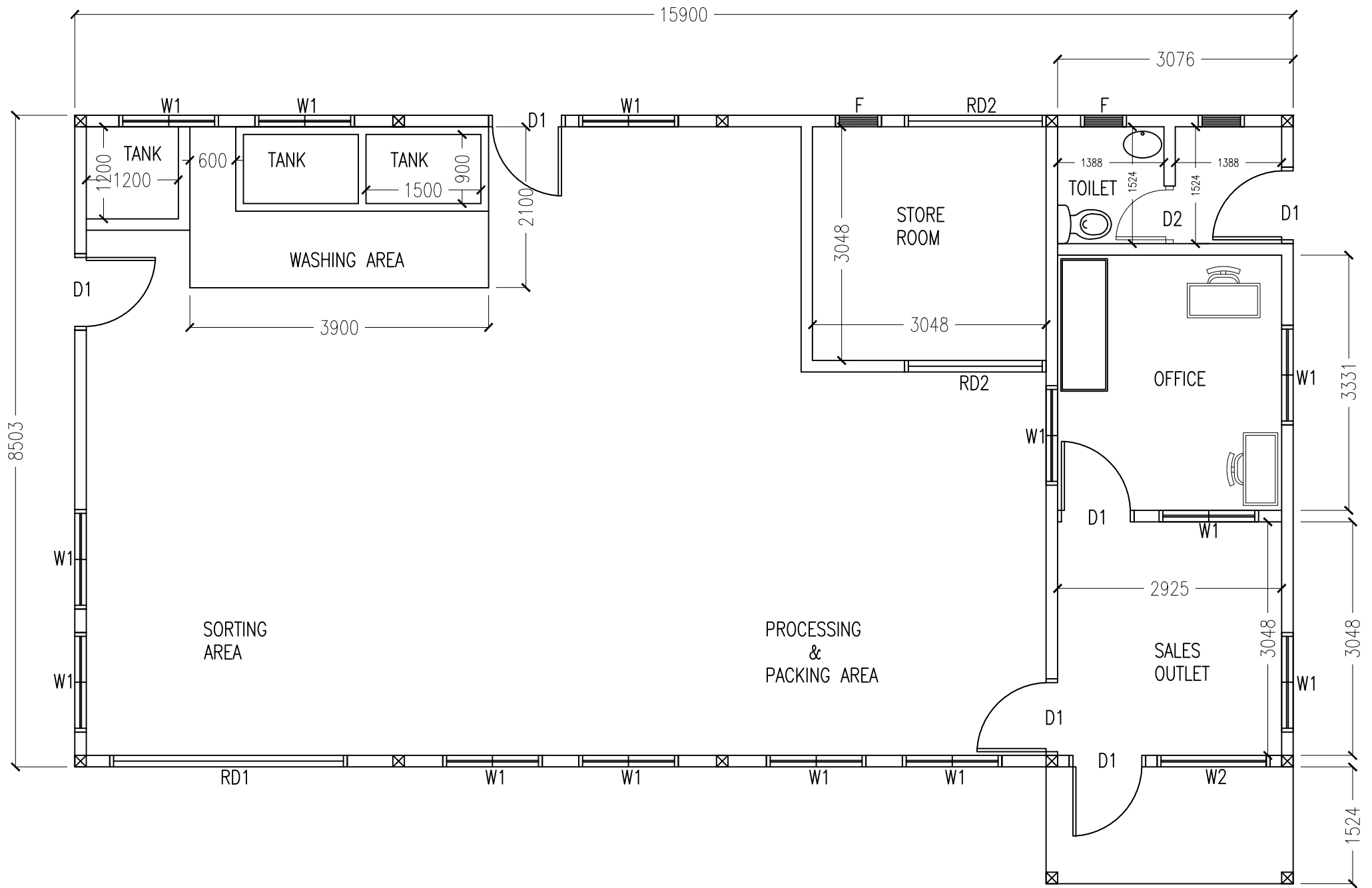
PROCESSING CENTER FLOOR PLAN
