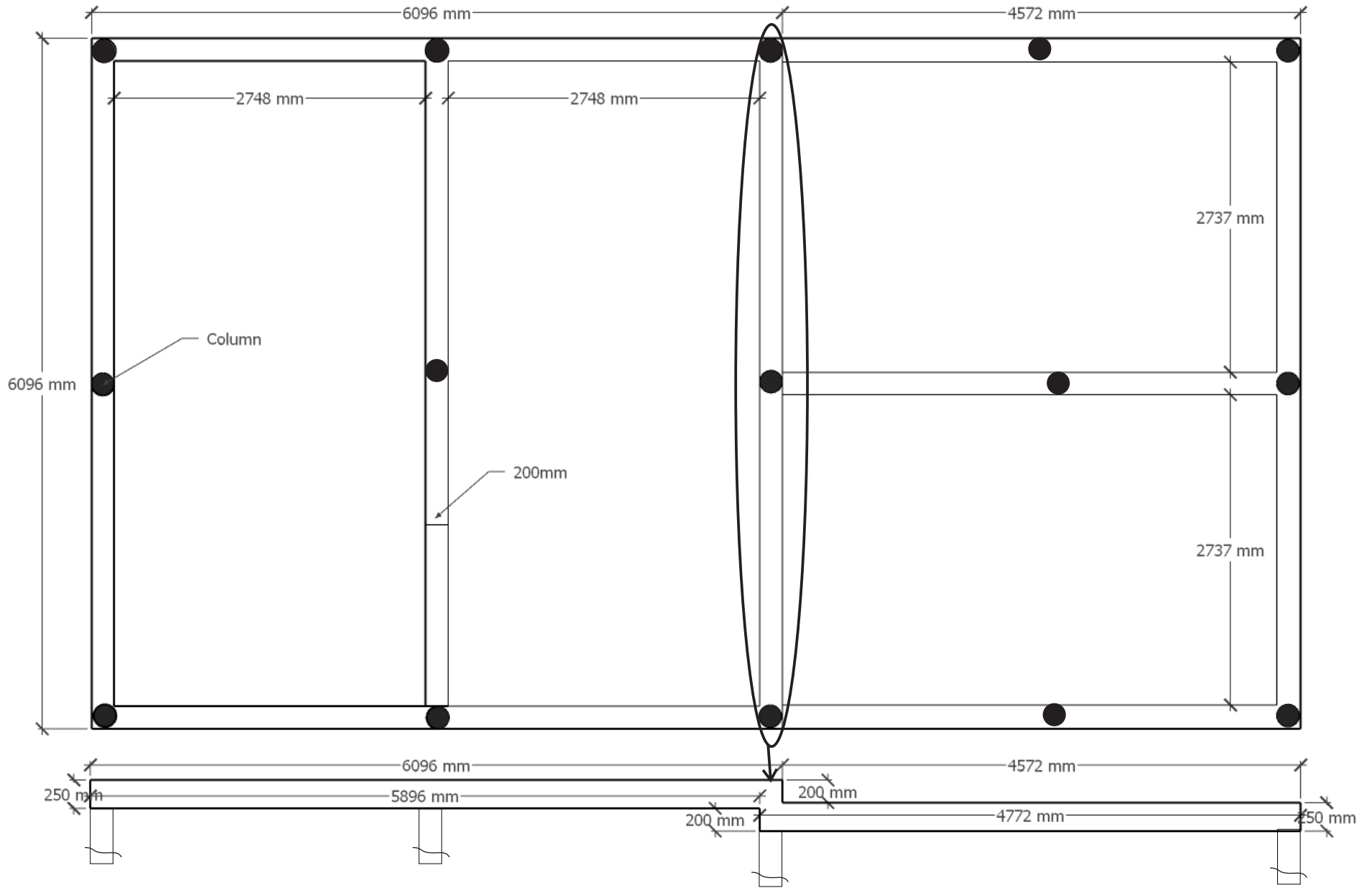
1 PLATFORM BEAM DETAIL A03 Not To Scale
