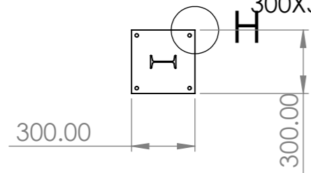
SECTION B-B SCALE 1 : 25 SB BEAM 8 NOS
