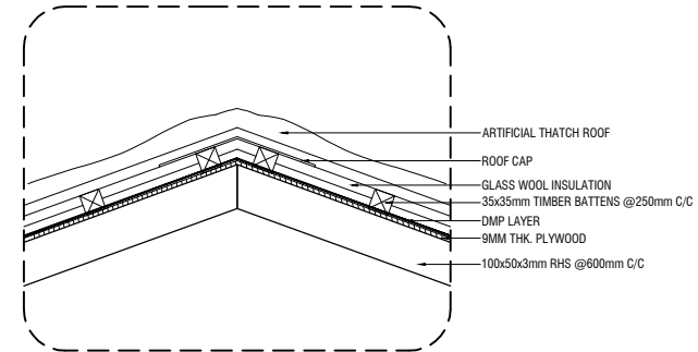
ROOFING DETAIL
